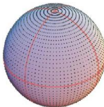
Figure 5: a) Geodesic ISEA4H grid of SMOS; b) regular latitude-longitude grid used for SM ECV
